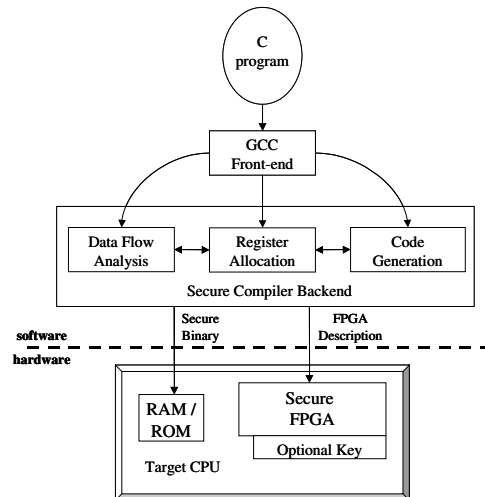
Figure 3. Compilation framework
