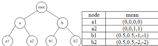
Figure 2: Description of the synthetic dataset
