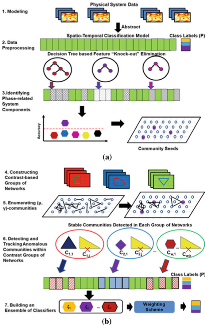
Fig. 4 The overview of our methodology. a Step 1–Step 3. b Step 4–Step 7
