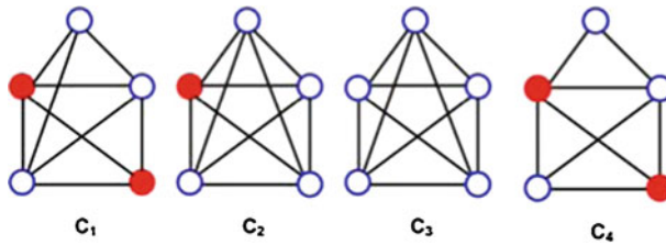
Fig. 1 An example of (\mu, \gamma) -communities. Filled nodes: seed nodes, empty nodes: normal nodes
