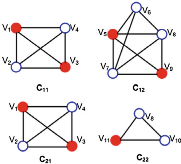
Fig. 3 An example of anomalous communities. C_{11} and C_{12} are conserved communities from the network group U_1 , and C_{21} and C_{22} are conserved communities from the network group U_2 . Filled nodes: seed nodes, empty nodes: normal nodes
