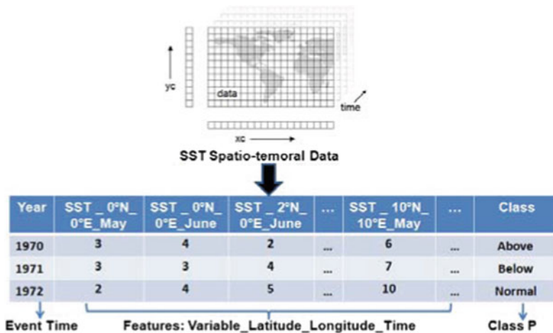
Fig. 5 Our proposed mathematical form for classification of spatio-temporal data
