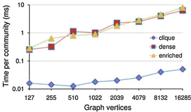
Fig. 9 Timing results for (\mu, \gamma) -community enumeration algorithm
