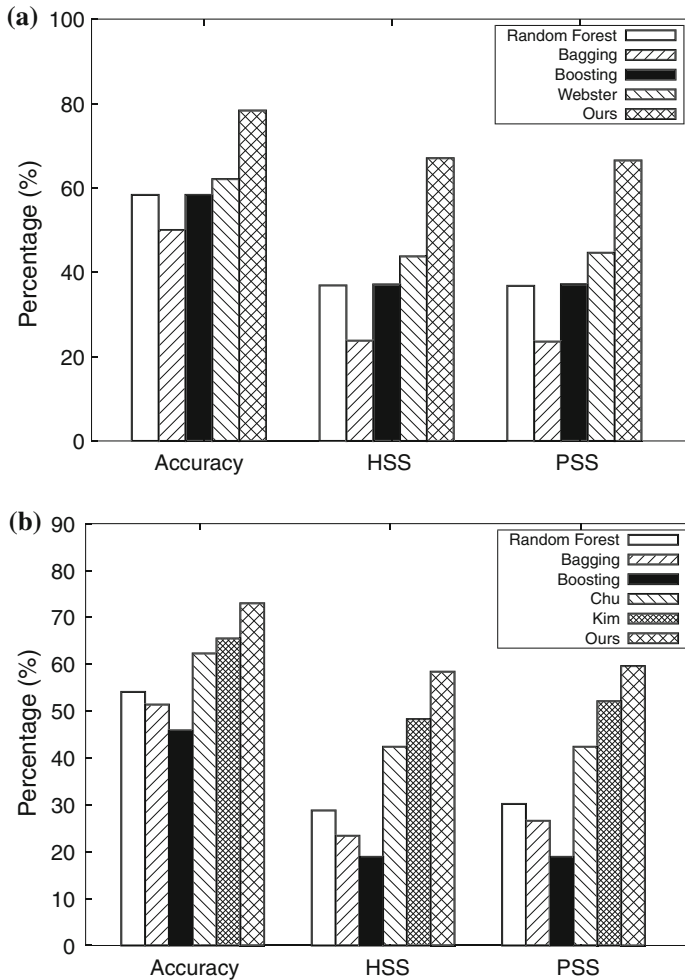
Fig. 8 LOOCV performance for seasonal TC prediction. a North Atlantic TC prediction. b North Pacific TC prediction
