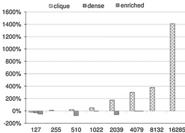
Fig. 10 Speedup results for using hierarchical bitmap index in (\mu, \gamma) -community enumeration algorithm
