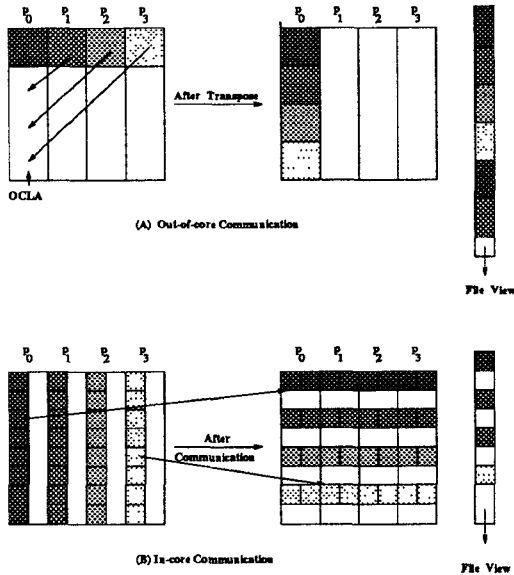
Figure 8: Out-of-core Transpose.
