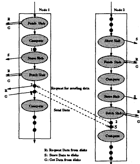
Figure 5: Demand-driven In-core Communication. Node 2 requests data from Node 1 (point 2). Node 1 reads data from disks and sends to node 2 (points 4-5).
