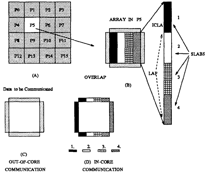
Figure 3: Figure illustrates compilation of out-of-core difference equation. The in-core slabs and the corresponding ghost areas are shown using distinct shades.
